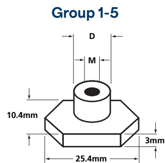
Rail Nut
