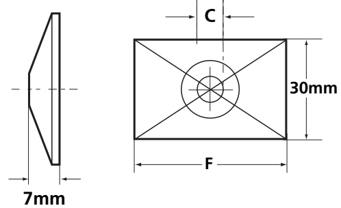
Cover Plate
