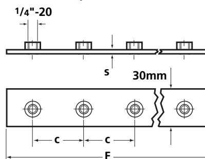
Multiple Weld Plate
