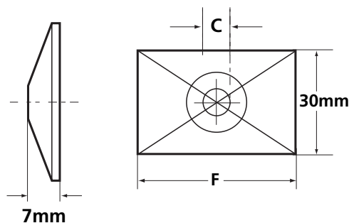
Cover Plate
